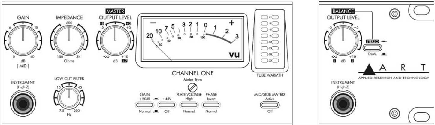
Figure 2 – Front controls
