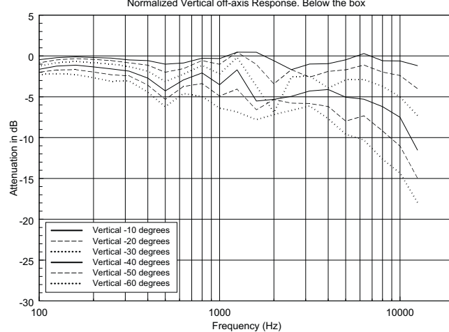
Normalized Vertical off-axis Response. Below the box
