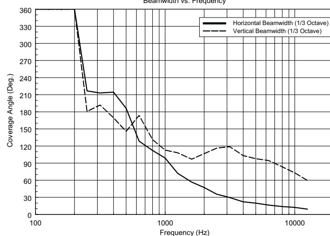
Beamwidth vs. Frequency
