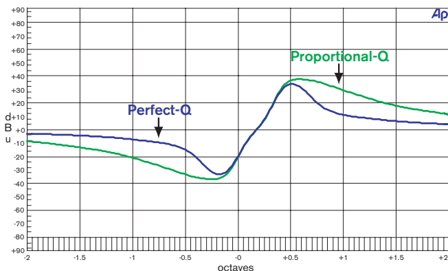
Figure 3. Phase response of Figures 1 and 2.
