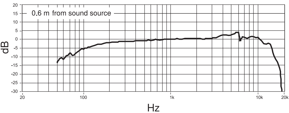
Frequency Response
