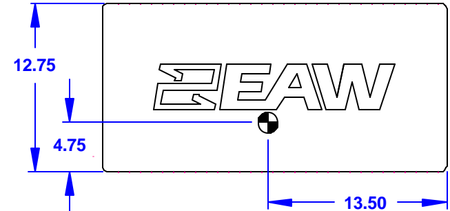
BACK
