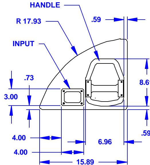
RIGHT SIDE
