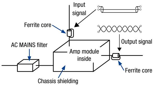
FIGURE 4: Tools and best practice for improving the electromagnetic compatibility.
