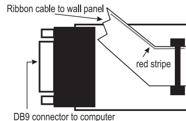
PROGRAMMING PORT
