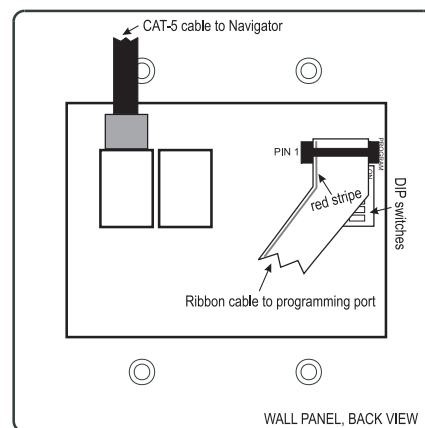
WALL PANEL, BACK VIEW
