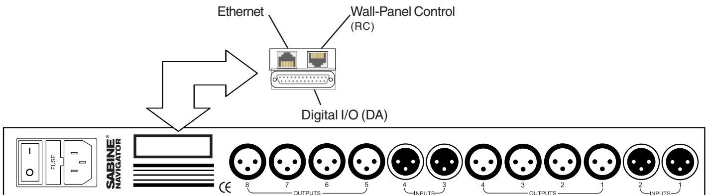
NAV4802 back panel, with DA option (DB25 Connector) and RC option (RJ45 connector)
