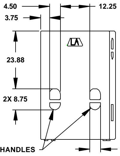
VIEW A-A DIMENSIONS APPLY TO BOTH SIDES
