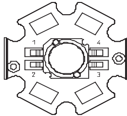
Figure 9. K2 Star Package Outline Drawing.
