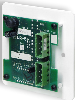
WR-5e European Version
