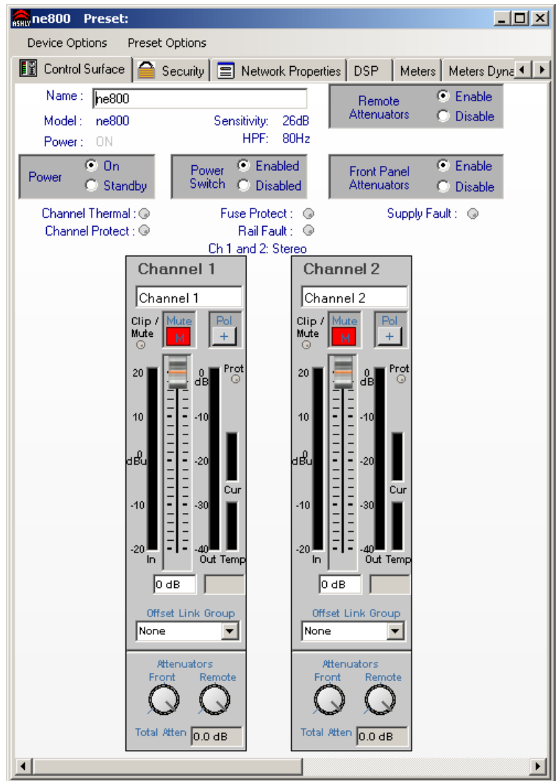
Protea ne Two-Channel Amplifier Control Surface
